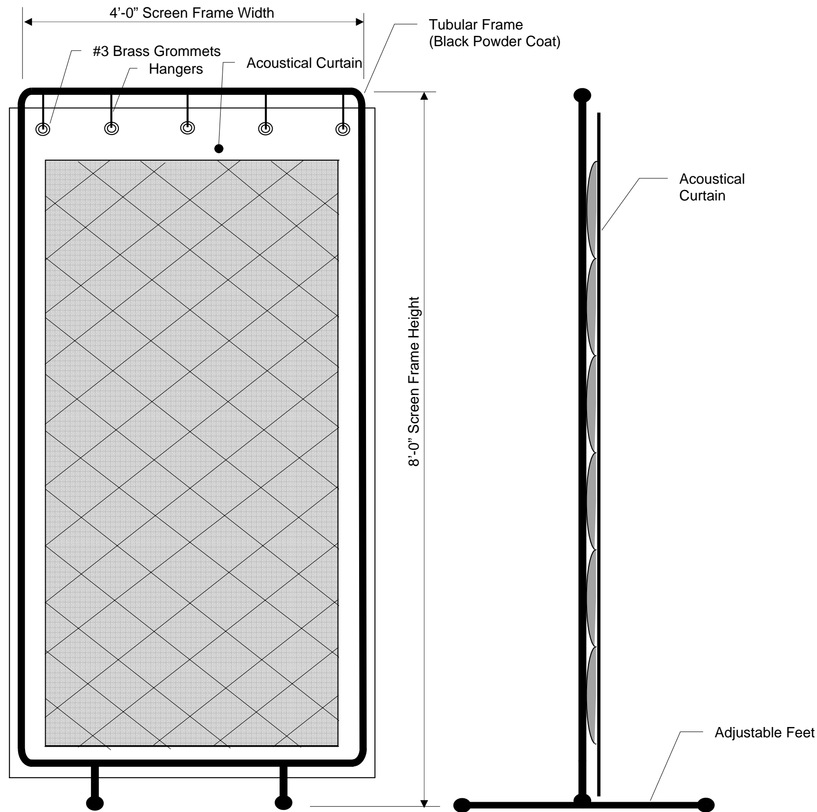
STANDARD SCREEN ASSEMBLY Shown With Composite Curtain
