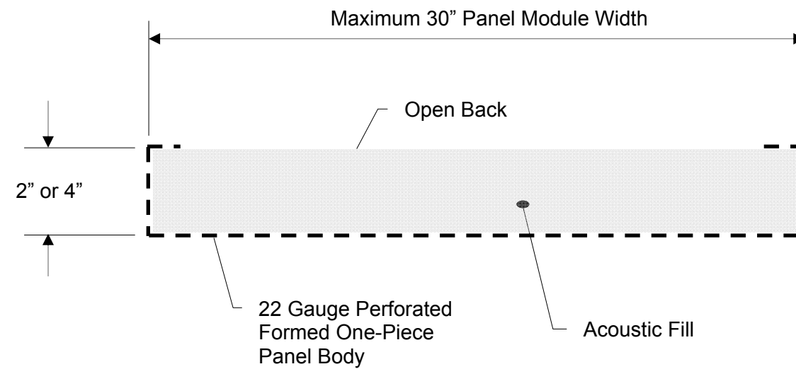
VIEW "A" STANDARD PANEL CONSTRUCTION
