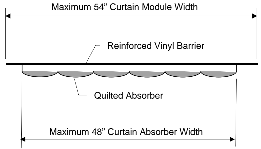
COMPOSITE CURTAIN (Barrier / Absorber)
