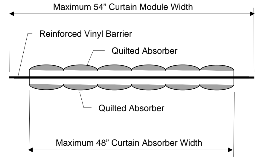
SEPTUM CURTAIN (Absorber / Barrier / Absorber)
