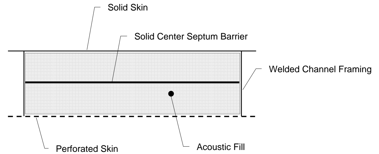
SUPER STC PANEL CONSTRUCTION (Barrier / Fill / Septum Barrier / Absorber)
