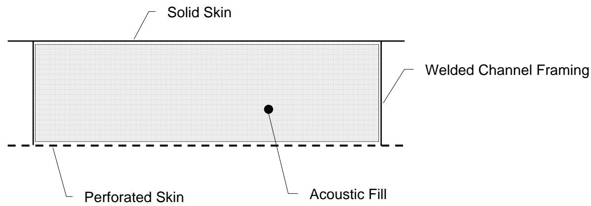
STANDARD PANEL CONSTRUCTION (Barrier / Absorber)
