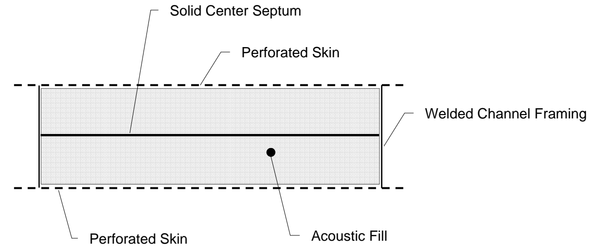
SEPTUM PANEL CONSTRUCTION (Absorber / Septum Barrier / Absorber)
