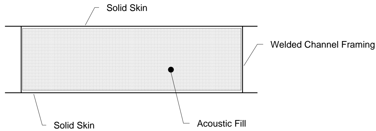
HARD PANEL CONSTRUCTION (Barrier / Barrier)
