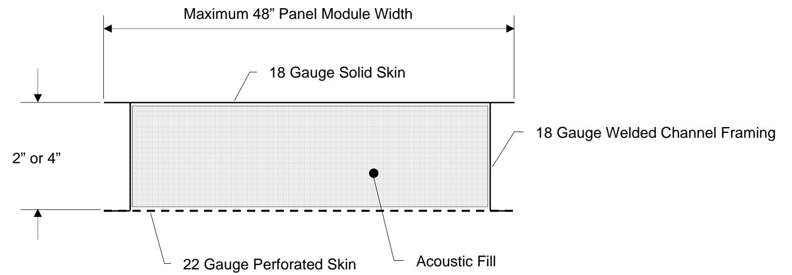
STANDARD PANEL CONSTRUCTION
